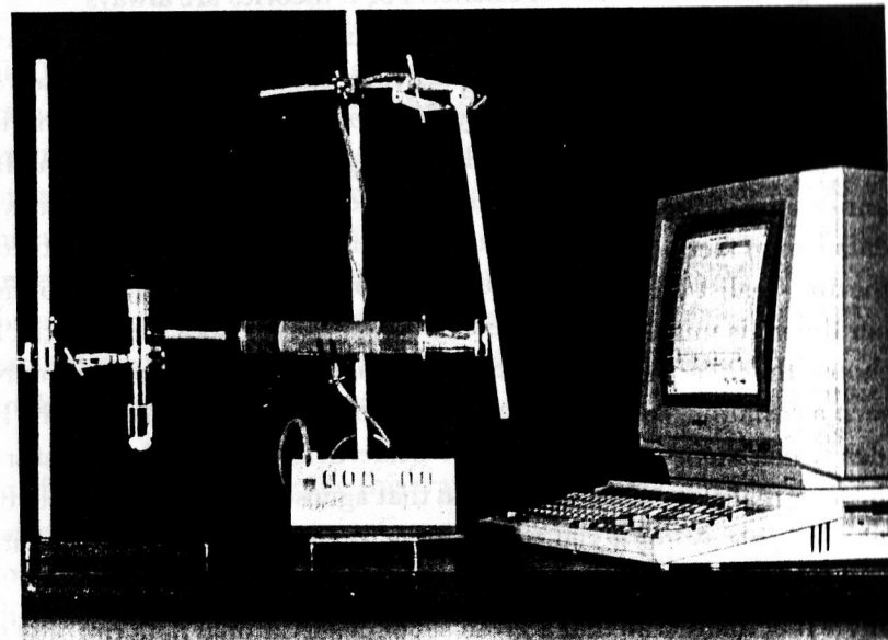
10. Dialometer for measuring the change in volume of a gas as its temperature varies.
